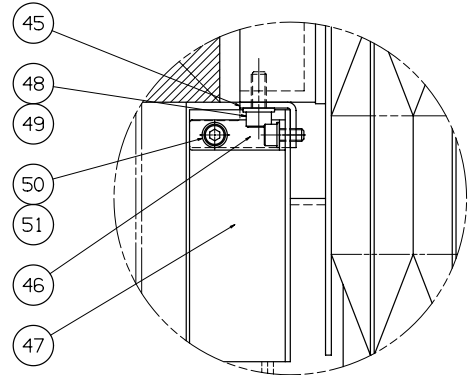
E DETAIL (S= 1/1)
