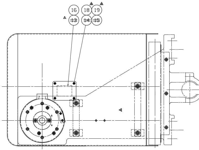
A VIEW
