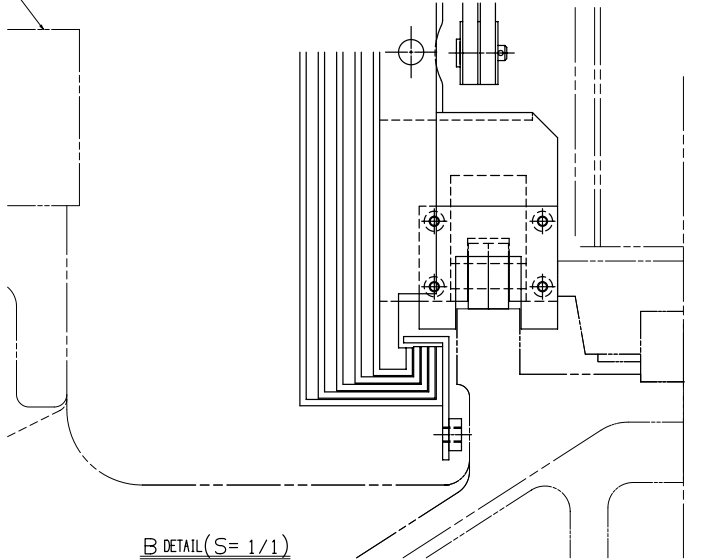
B DETAIL(S= 1/1)
