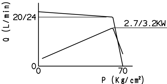
ホンプ性能曲線(50/60Hz) (PUMP CHARACTERISTIC CURVES)
