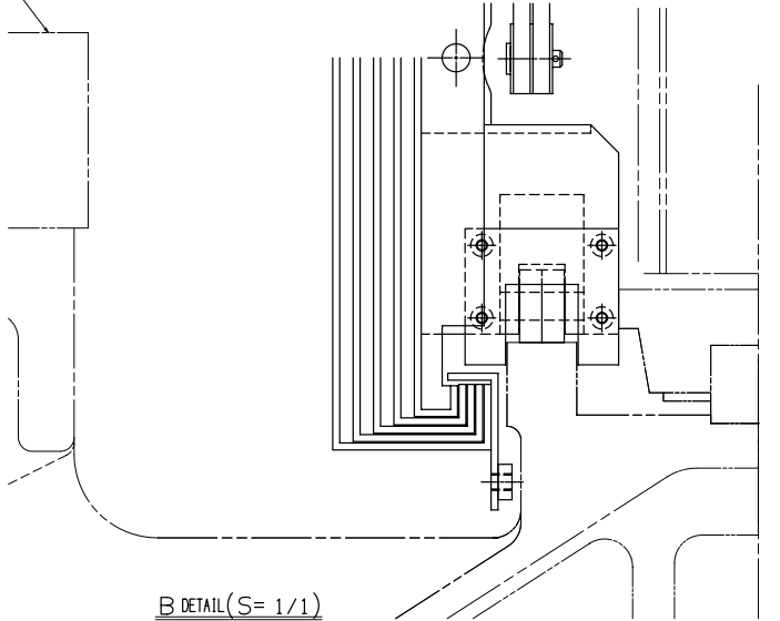
B DETAIL (S= 1/1)
