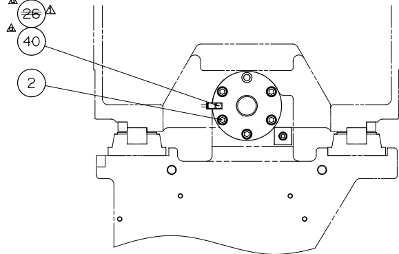
B-SECTION
