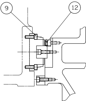
A - A SECTION (S=1/2)
